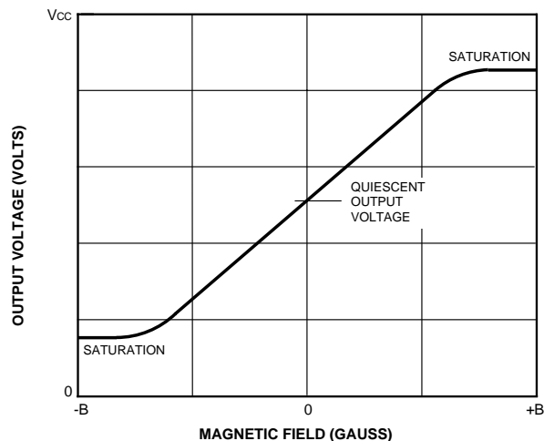
Linear Sensor Characteristic
