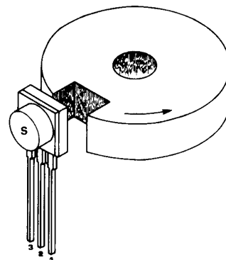
Biased Linear Sensing for Notch Detection
