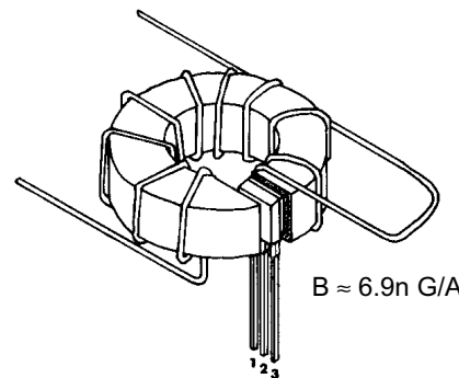
Multiple Turns for Measuring Low Currents
